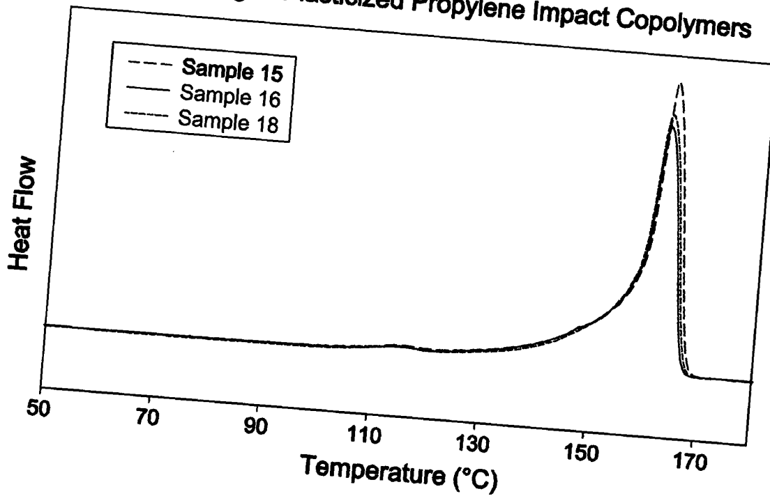
Fig. 10 DSC Crystallization of Plasticized Propylene Impact Copolymers
